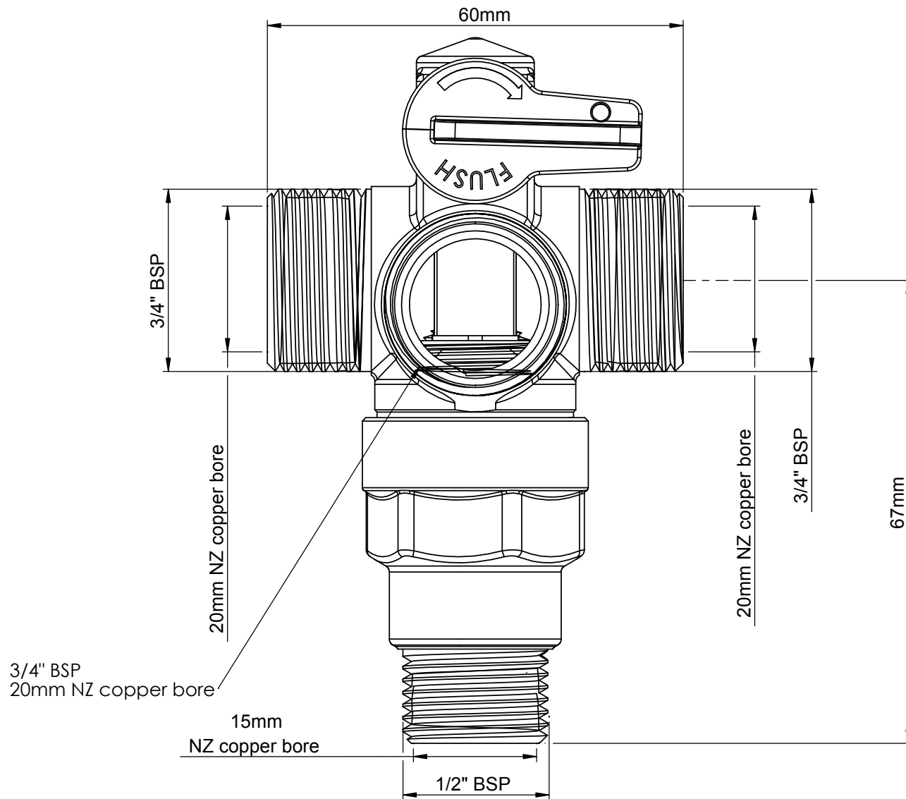
Cold water expansion valve (EVT low pressure)
